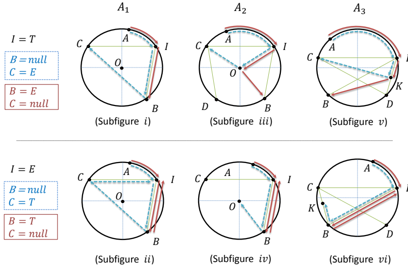
Figure 5: The non-wireless algorithm for two robots with performance \pi - \alpha/2 + 3 \sin(\alpha/2) .
