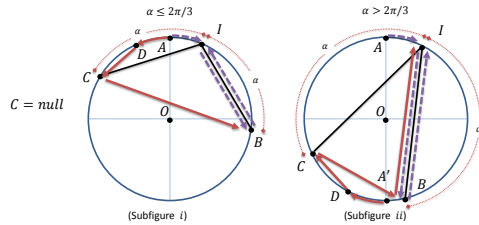
Figure 3: The performance of the wireless algorithm, when the starting point A lies outside the arc 5.0\text{pt}\widehat{IB} of the two interesting points. The trajectory of R_2 is depicted with the dotted purple curve, while the trajectory of R_1 with the solid red curve.
