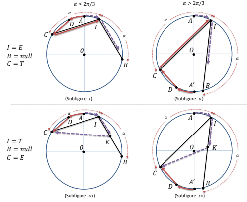
Figure 2: The performance of the wireless algorithm, when the starting point A lies in the arc 5.0\text{pt}\widehat{CI} of the two interesting points. The trajectory of R_2 is depicted with the dotted purple curve, while the trajectory of R_1 with the solid red curve.
