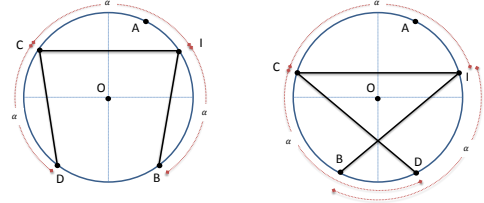
Figure 4: The points of interest from the perspective of R_2 , when \alpha \leq 2\pi/3 on the left, and when \alpha \geq 2\pi/3 on the right.
