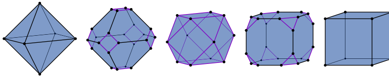
FIGURE 2. The polytope \rho_{3,k}^* , when k is equal to 1, 3/2 , 2, 5/2 , and 3 (from left to right).
