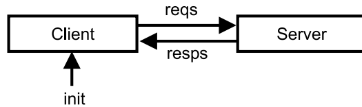
Figure 2: Client-Server Simulation
