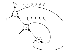
Figure 1: Circular Fibonacci Sequence
