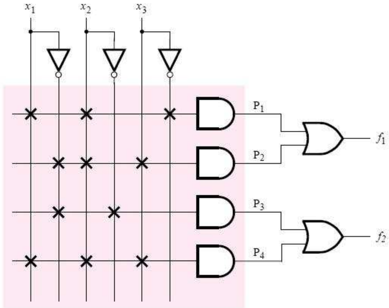
AND plane
