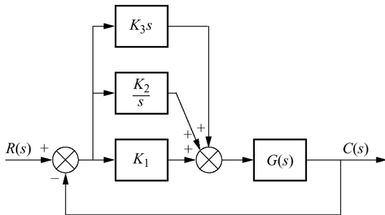
Figure 9.30: PID Controller.
