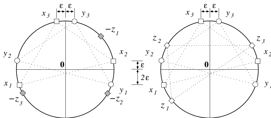
FIGURE 4. Valid minimal configuration \mathbf{S}^- in dimension 2 with \mathbf{depth}_{\mathbf{S}^-}(\mathbf{0}) = 5 .
