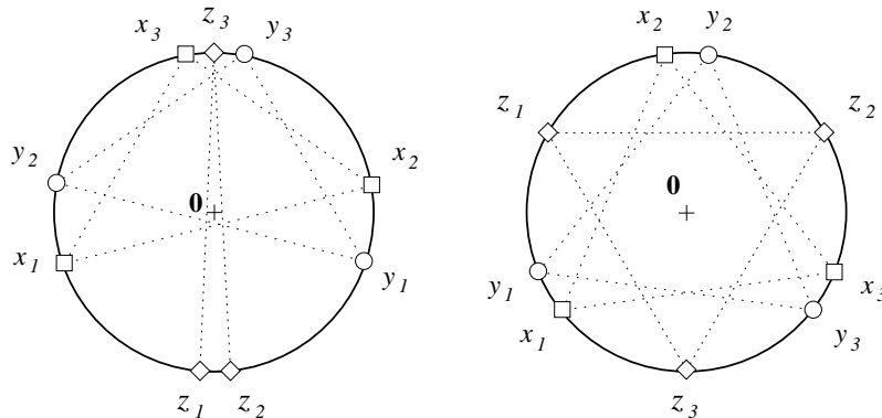
FIGURE 5. The two valid minimal configurations in dimension 2 with \mathbf{depth}_{\mathbf{S}}(\mathbf{0}) = 9 .
