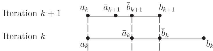
Figure 4.3: Illustration of consecutive iterations of the Golden section rule when \phi(\bar{a}_k) < \phi(\bar{b}_k) .
