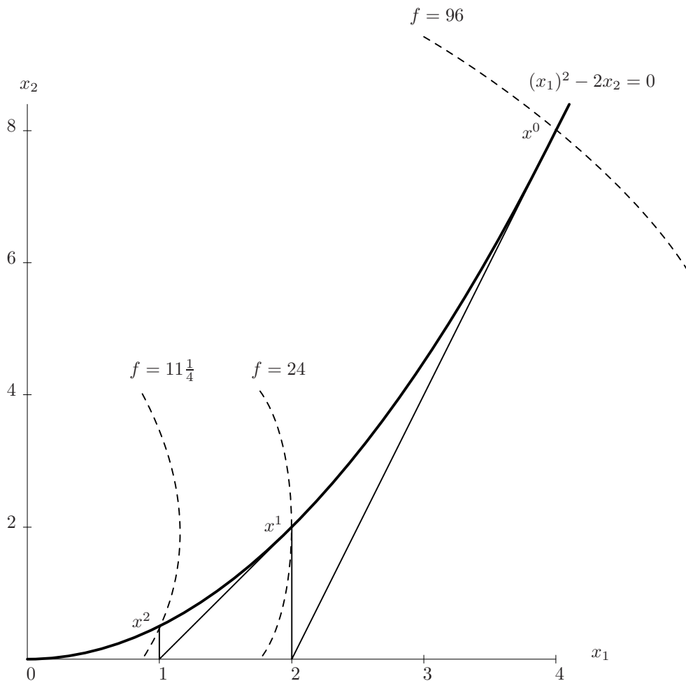
Figure 5.1: Illustration of Example 5.6.
