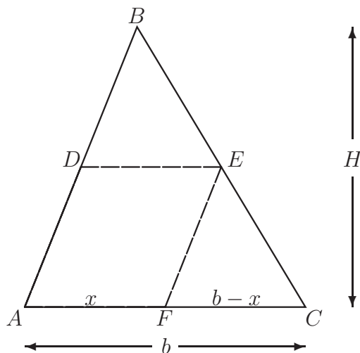
Figure 2: Illustration of Euclid's problem.
