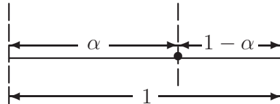
Figure 4.1: The golden section: \alpha \approx 0.618 .
